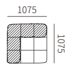
SE05E-1 1075*1075*680MM 42.3*42.3*26.8"
