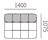
SE05B-2 1400*1075*680MM 55.1*42.3*26.8"
