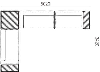
HW03E-1 + HW03AB-4R + HW03E-3 + HW03A-4R + HW03B-2 + HW03F-2 5020*3420*660MM 197.6*134.6*26.0"
