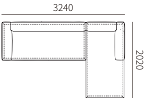
HW03A-6R + HW03C-2L 3240*2020*660MM 127.6*79.5*26.0"
