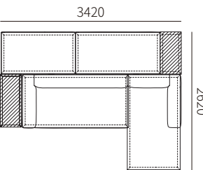
HW03D-1 + HW03D-2 + HW03F-1 + HW03E-1 + HW03AB-4R + HW03C-1L 3420*2620*660MM 134.6*103.1*26.0"
