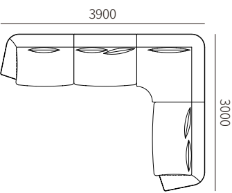
31F006-22R + 31F006-32 + 31F006-61 + 31F006-23L 3900*3000*790MM 153.5*118.1*31.1"
