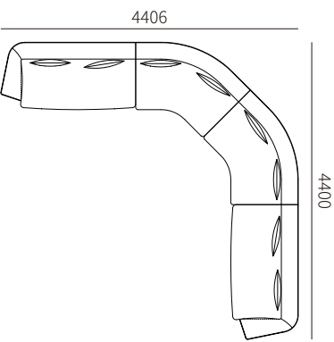
31F006-24R + 31F006-34*2 + 31F006-24L 4406*4400*790MM 173.5*173.2*31.1"
