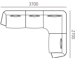
31F006-22R + 31F006-31 + 31F006-61 + 31F006-22L 3700*2700*790MM 145.7*106.3*31.1"
