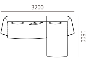
31F006-24R + 31F006-41L 3200*1800*790MM 126.0*70.9*31.1"
