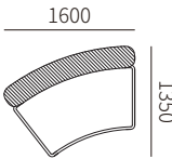
31F030-36 1600*1350*680MM 63.0*53.1*26.8"
