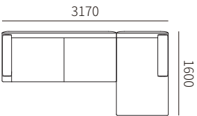
31F017-27R + 31F017-41L 3170*1600*690MM 124.8*63.0*27.2"
