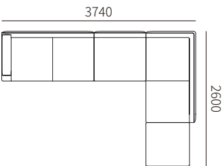
31F017-25 + 31F017-32 + 31F017-62 + 31F017-51 3740*2600*690MM 147.2*102.4*27.2"
