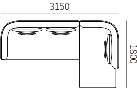
31F011-23R + 31F011-41L 3150*1800*680MM 124.0*70.9*26.8"
