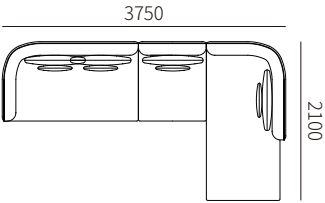
31F011-22R + 31F011-31 + 31F011-42L 3750*2100*680MM 147.6*82.7*26.8"
