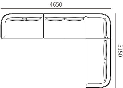
31F011-22R + 31F011-33 + 31F011-61 + 31F011-23L 4650*3150*680MM 183.1*124.0*26.8"
