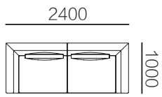
31F009ZH-01 2400*1000*680mm 94.5*39.4*26.8"
