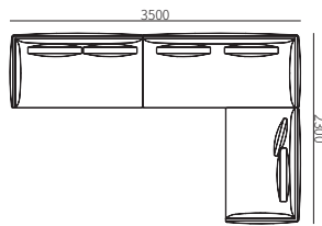
31F012ZH-05 3500*2300*680mm 137.8*90.6*26.8"
